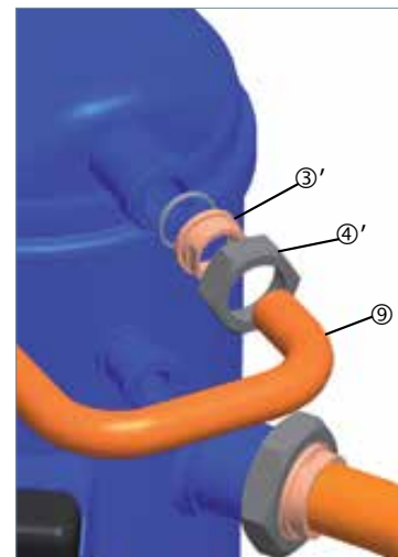
Discharge line
